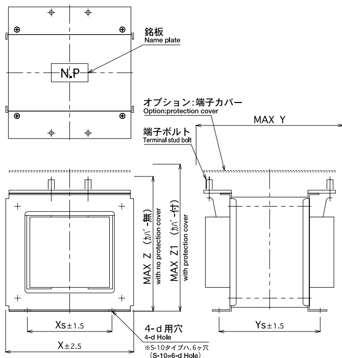
■取付穴図 (Mounting hole figure)
